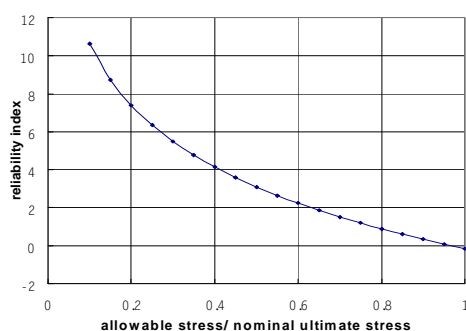
Figure 3. Reliability vs. Stress Ratio
