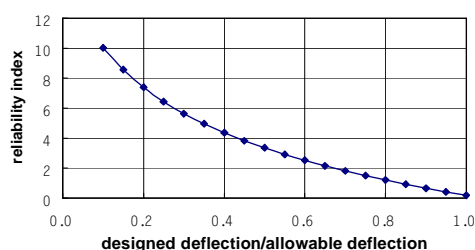
Figure 4. Reliability vs. Deflection Ratio
