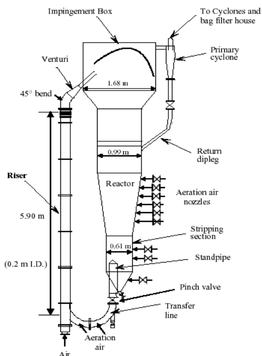
Figure 1 Schematic of fluid coker cold model with riser
