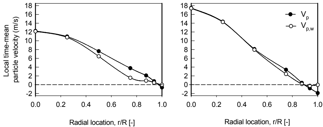
Figure 2 Comparison of radial profiles of time-average and concentration weighted time-mean particle velocities for U_g = 6 m/s and G_s \approx 340 kg/m 2 s at (a) z = 0.76 m; (b) z = 3.1 m.
