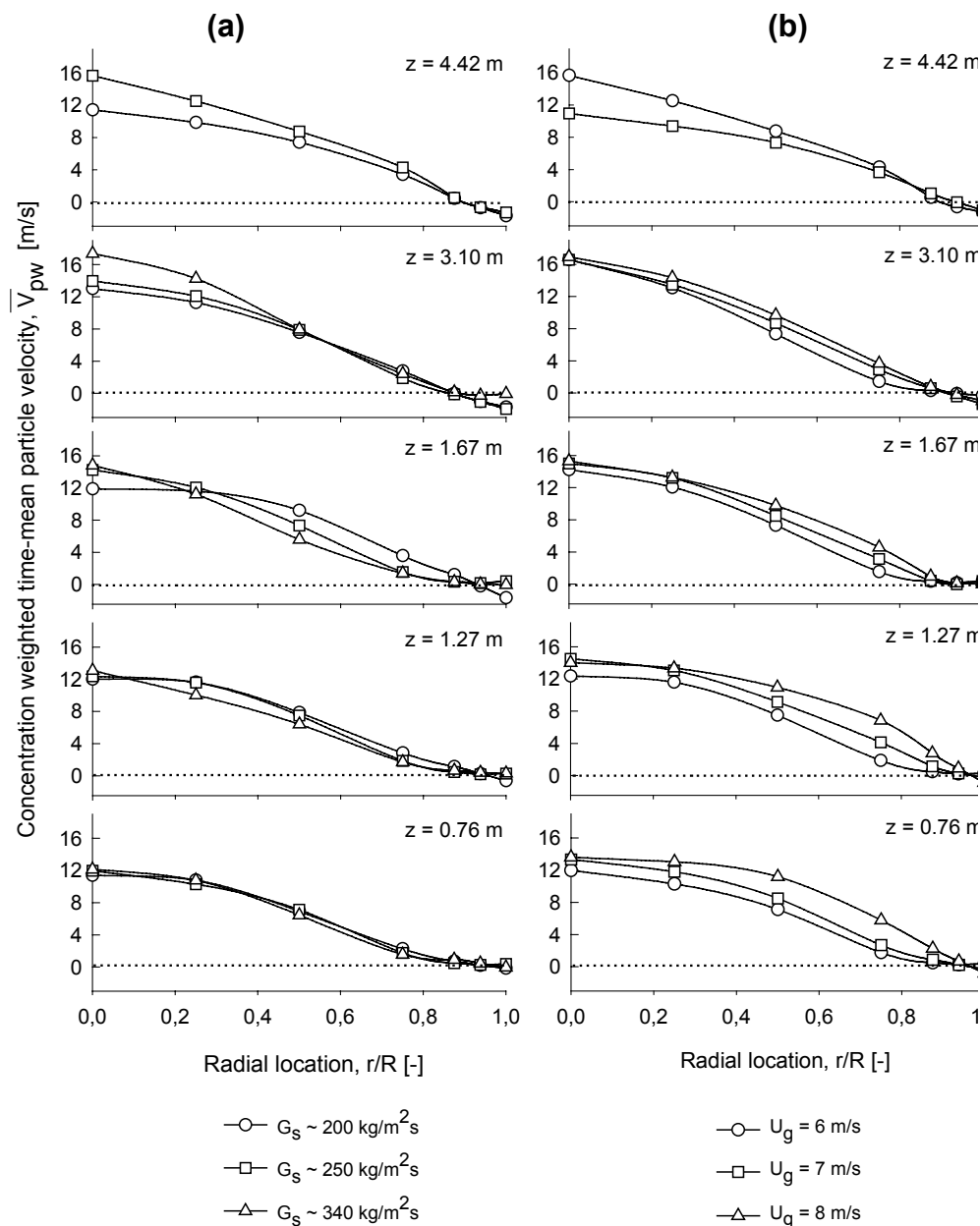
Figure 4 Local concentration-weighted time-mean particle velocity profiles at different axial locations for: (a) U_g = 6 m/s and various solids circulation fluxes (b) G_s \sim 250 kg/m 2 s and various superficial gas velocities
