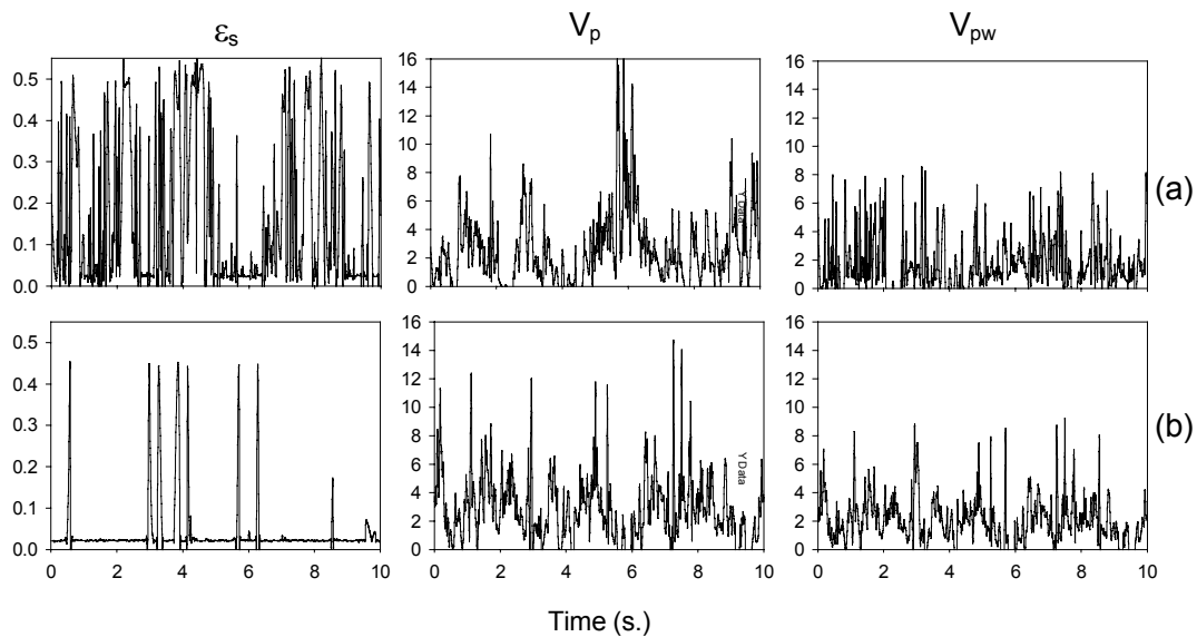
Figure 3 Instantaneous solids hold-up, particle velocity and concentration-weighted time-mean particle velocities for U_g = 6 m/s and G_s \sim 340 kg/m 2 s measured at r/R = 0.75 and at (a) z = 0.76 m and (b) z = 3.1 m.
