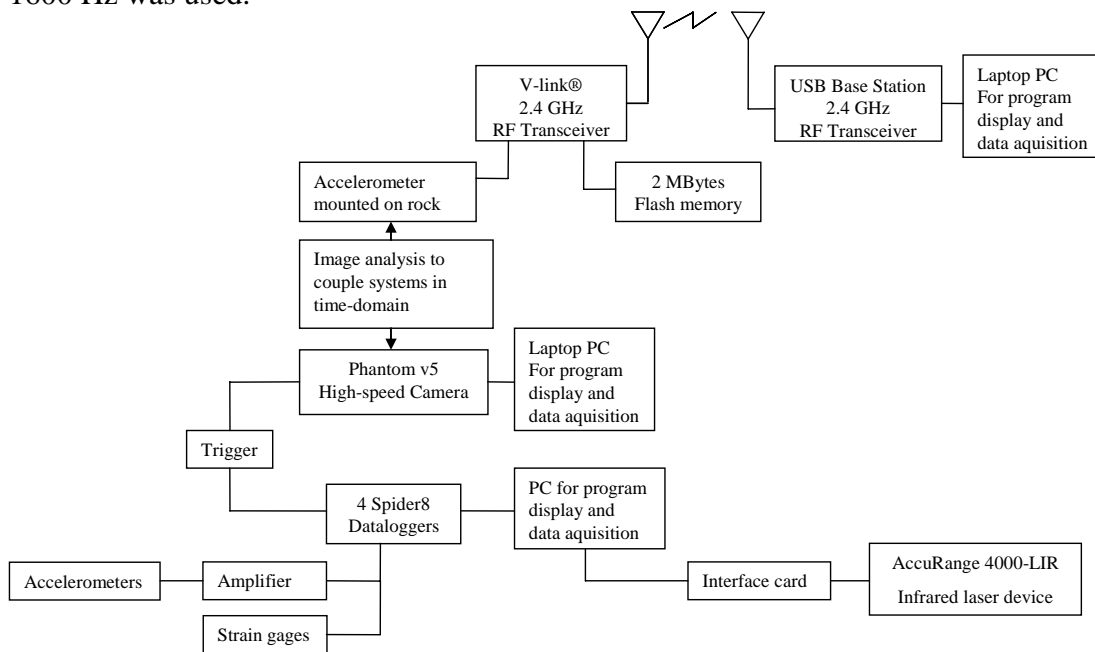
Figure 4: Schematic layout of data acquisition system.
