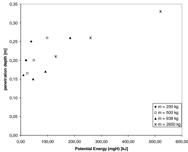
Figure 5: Penetration depth vs Energy for rockfall tests with rock masses of 200, 500, 938 and 2650 kg. Fall heights varying from 5, 10 and 20m.
