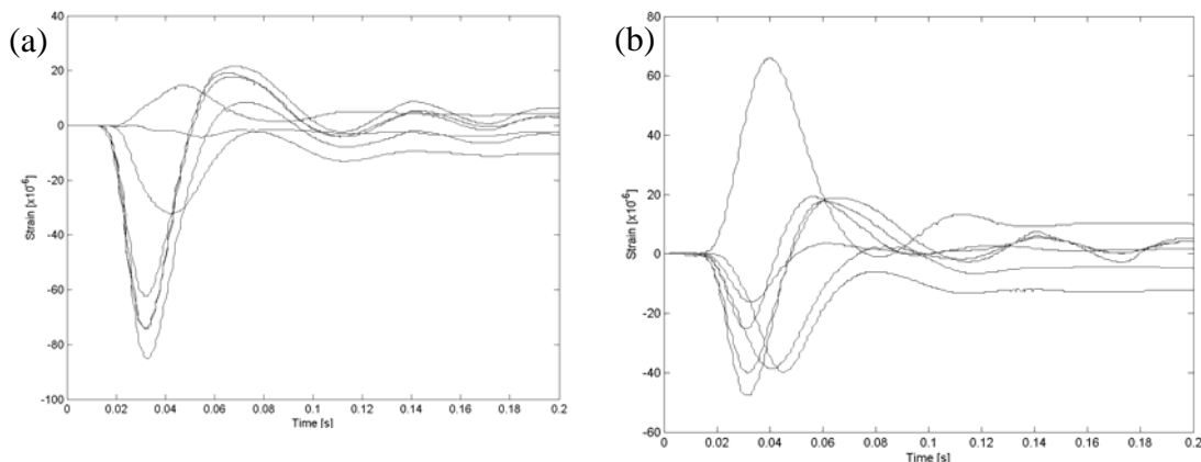
Figure 8: (a) Measured axial strains for the culvert at profile P2 during impact and (b) bending strains for the culvert at profile P2 during impact.
