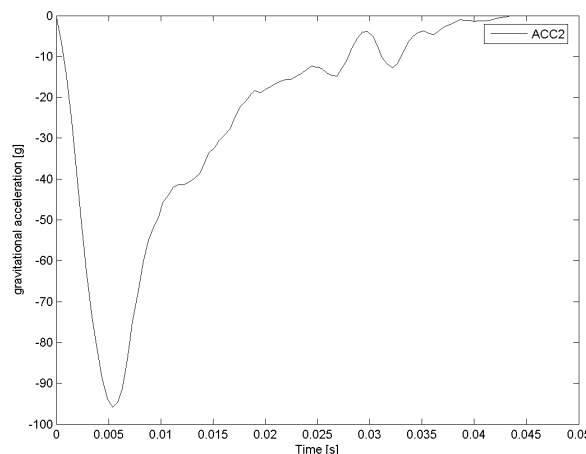
Figure 6: Typical deceleration history of low-energy rockfall impact.
