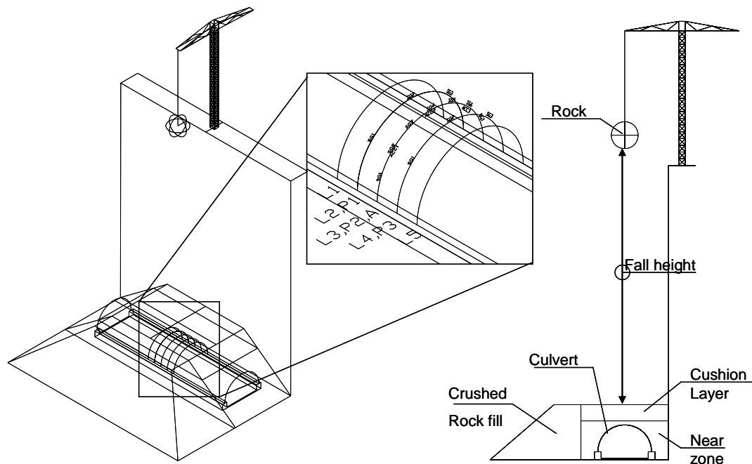
Figure 1: Illustration of experimental setup. Inset shows the different profiles where measurements were carried out.
