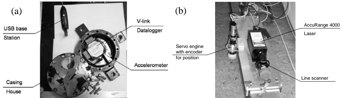
Figure 2: (a) Accelerometer device used to acquire deceleration history of rock impact, (b) laser device used to detect deformations of the culvert.
