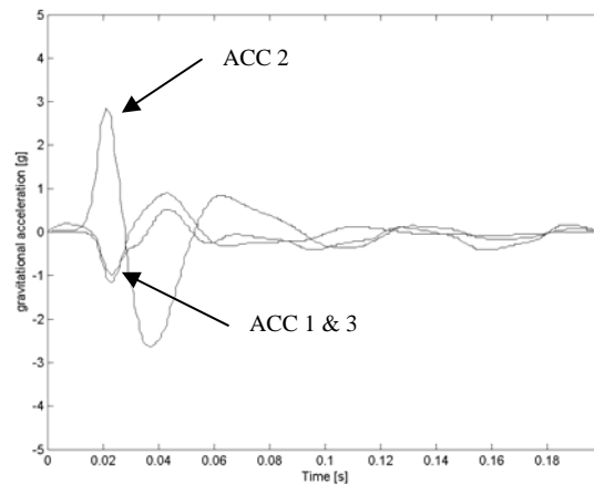
Figure 7: Measured accelerations in the culvert at profile S2 during impact.
