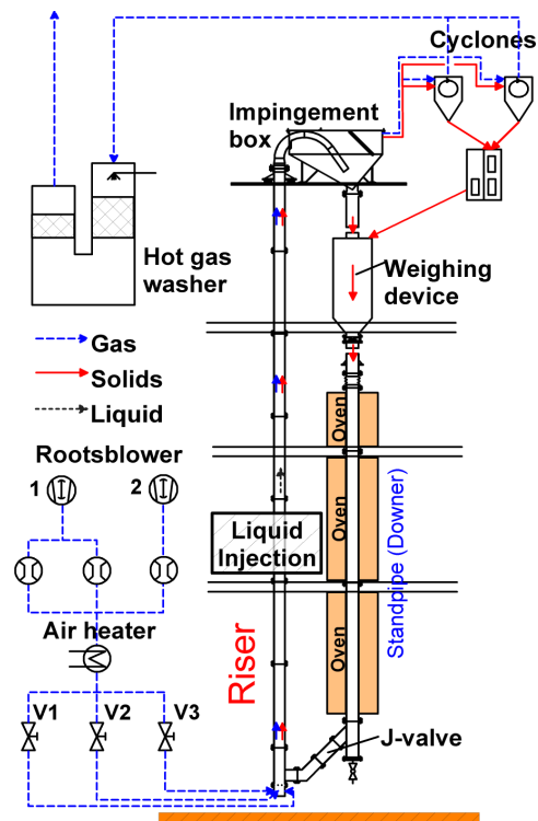
Figure 1: Experimental setup
