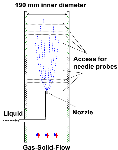
Figure 2: Injection geometry (axial)
