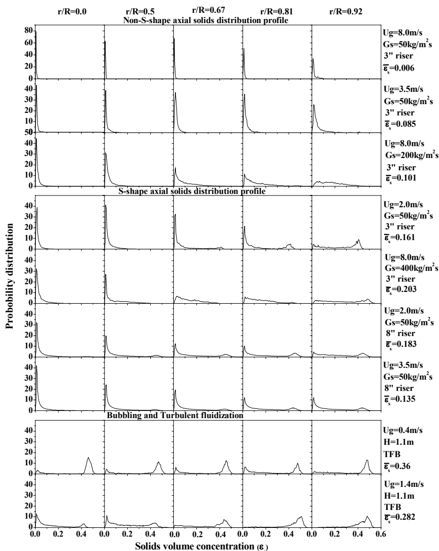
Fig.6 Comparison between the probability density distribution of local solids concentration in bottom region of CFB and TFB
