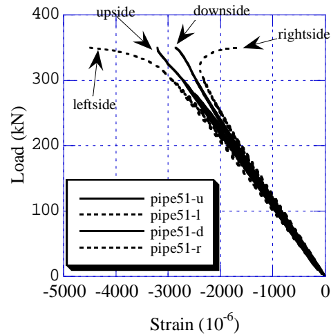
Fig.14 Upper Chord Load/Strain Relationship
