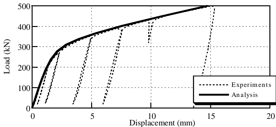
Fig.12 Load/Displacement Relationships
