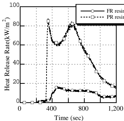
Fig.6 Relationships between Heat Release Rate and Time
