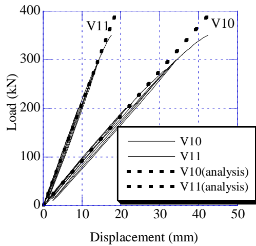
Fig.13 Load/Displacement Relationship
