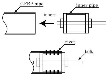
Fig.10 Joint Structure
