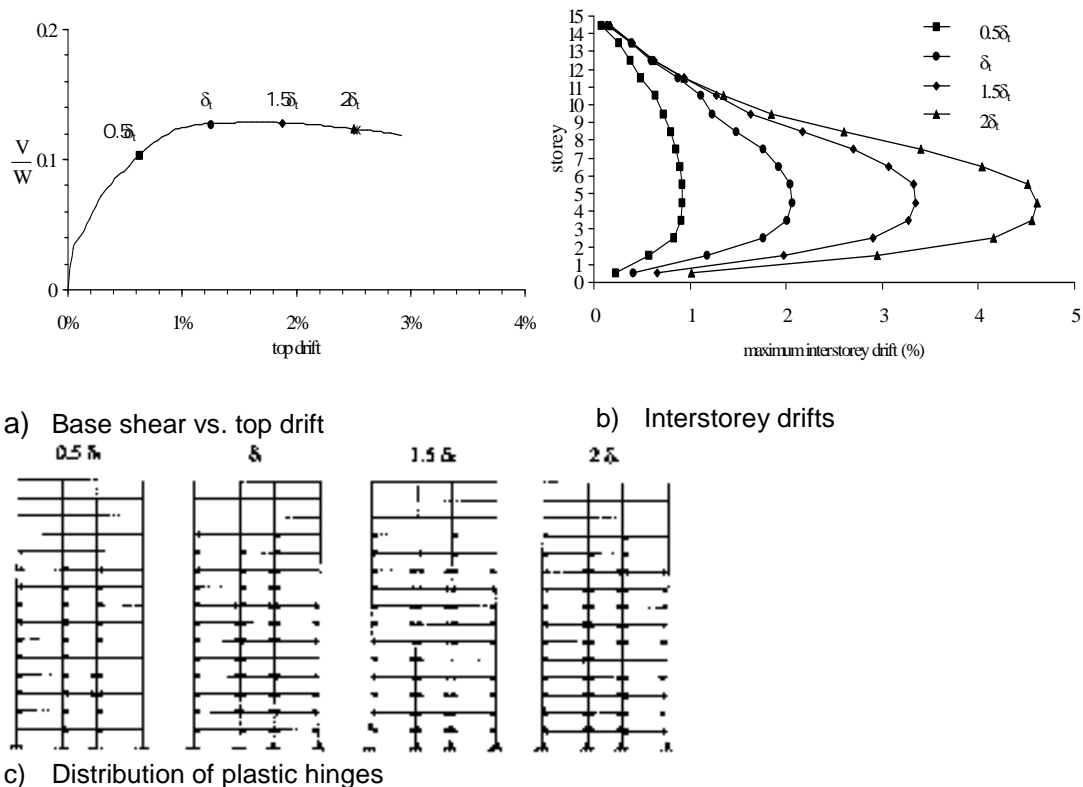
Figure 2. Pushover analysis results for f_c 50 f_y 500 -H building
