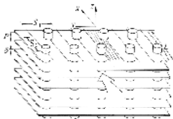
Fig. 1 Pictorial view of a plain plate tube-and-fin surface.
