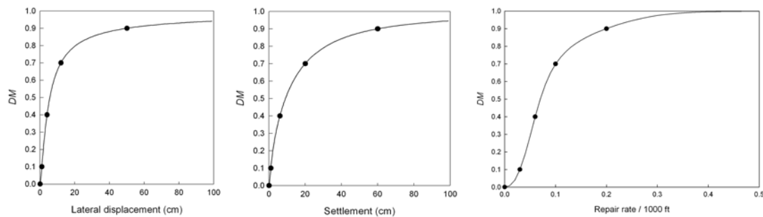
Figure 2. Graphical illustration of damage models: (a) slope instability and lateral spreading, (b) settlement, and (c) buried pipeline damage. Solid circles mark boundaries between different damage levels.
