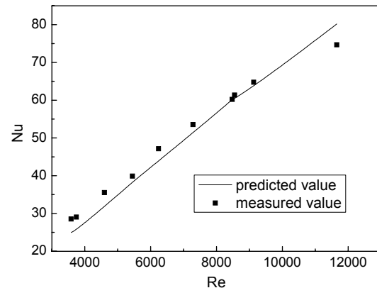
Fig.3 Shell-side heat transfer Nusselt number vs. Reynolds number
