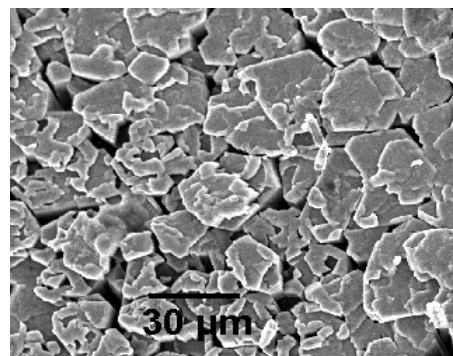
Fig. 3 Bare surface with surface energy 39.6 mN/m
