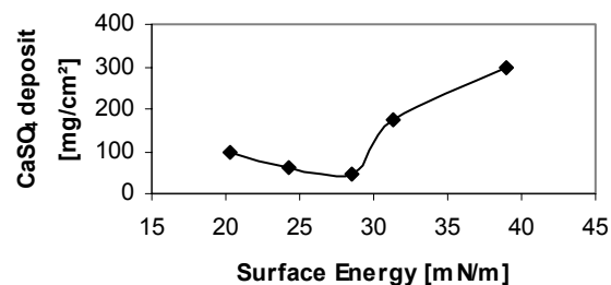
Fig. 2 Effect of the surface energy of the coatings on the adhesion of CaSO 4 deposits
