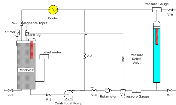
Fig. 3 Recirculating loop
