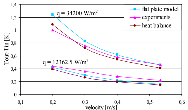
Fig. 8. Temperature difference between the inlet and outlet of the experimental setup and the flat plate geometry model achieved with the Heat flux boundary condition as a function of velocity.
