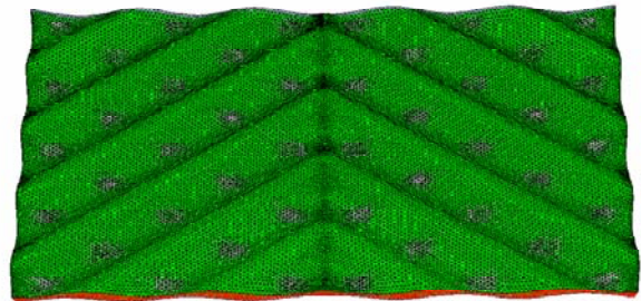
Fig. 1. 3D corrugated plate heat exchanger geometry with a computation mesh.
