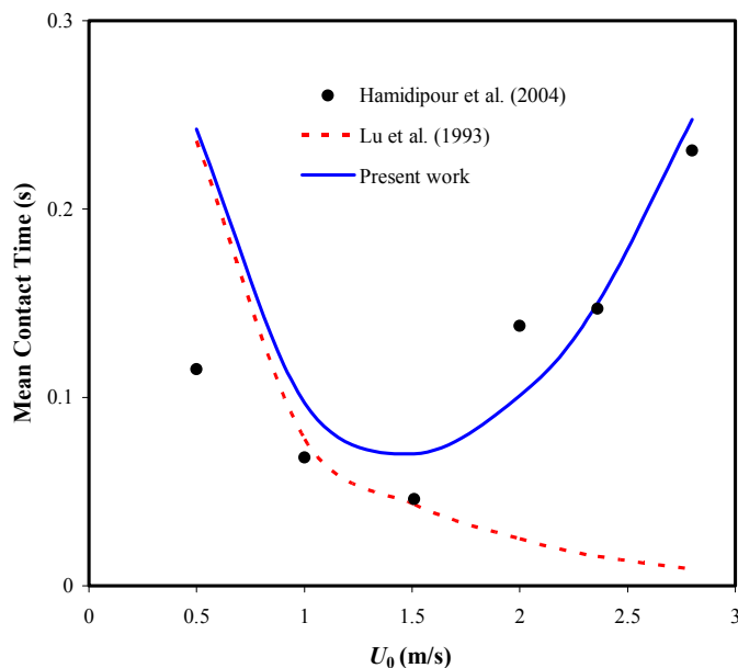
Figure 4 Variation of particle residence time as a function of superficial gas velocity, Sand particles
