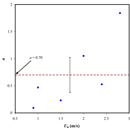
Figure 2 Existence probability ratio of bubble near wall and in the bed ( a_{ave}=0.70 ).
