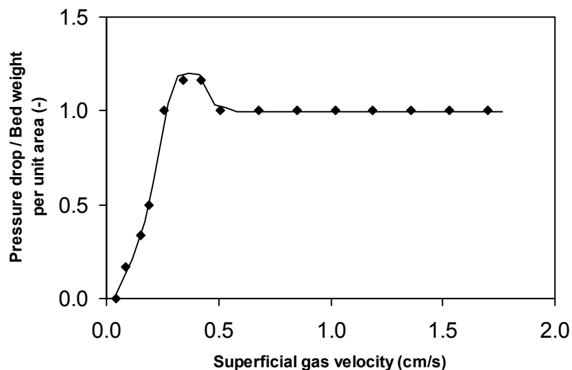
Fig. 2 Variation of bed pressure drop as a function of increasing superficial gas velocity (even packing; static bed height = 25 mm).
