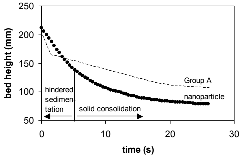
Fig. 4 Example of bed collapse after fluidizing gas was turned off (static bed height = 75 mm).
