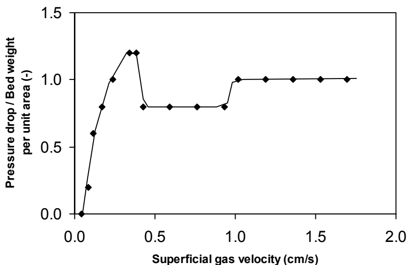
Fig. 3 Variation of bed pressure drop as a function of increasing superficial gas velocity (uneven packing; static bed height = 17.5 mm).
