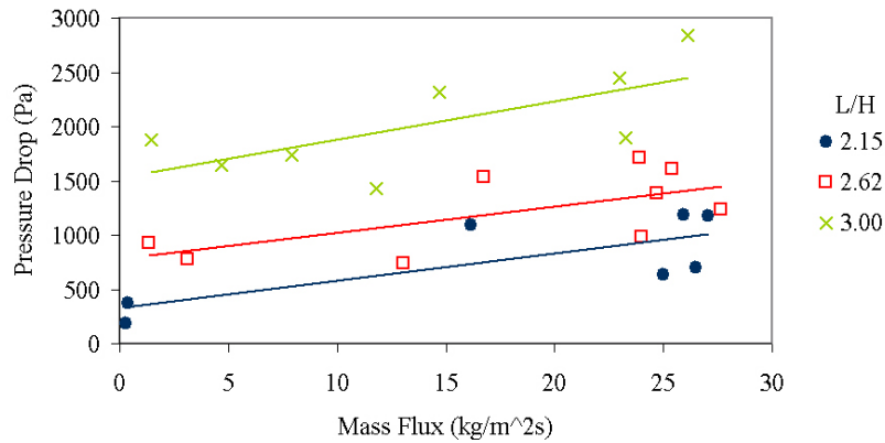
Figure 4: Pressure drop across the horizontal passage increases with solid mass flux and passage length.
