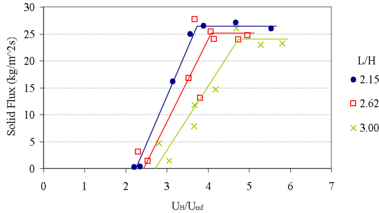
Figure 3: Changing Solid Flux with Supply Chamber Aeration and Horizontal Passage Length
