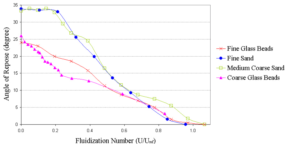
Figure 2: Variation in angle of repose/friction against aeration velocity with different particles
