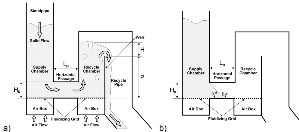
Figure 1: a) Loop seal set-up with finite passage length as used in current work. b) Angle of repose of sand and angle of sand required before sand can be recycled
