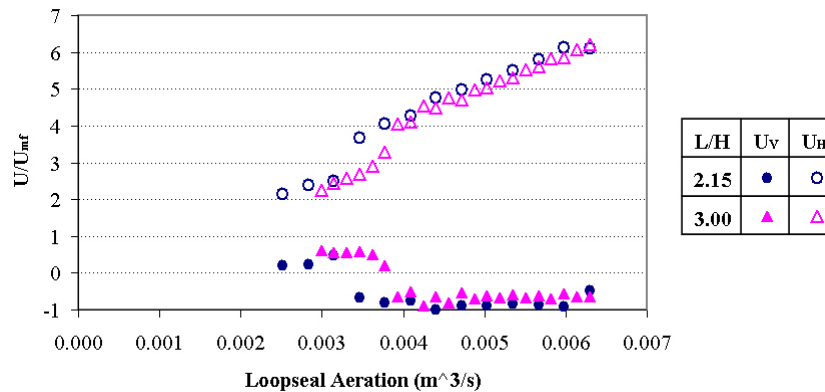
Figure 5: Split of aeration velocity ( U/U_{mf} ) between supply chamber and horizontal passage. Here U_V is the velocity of gas flowing up through the standpipe and U_H is the velocity of gas passing through the horizontal passage.
