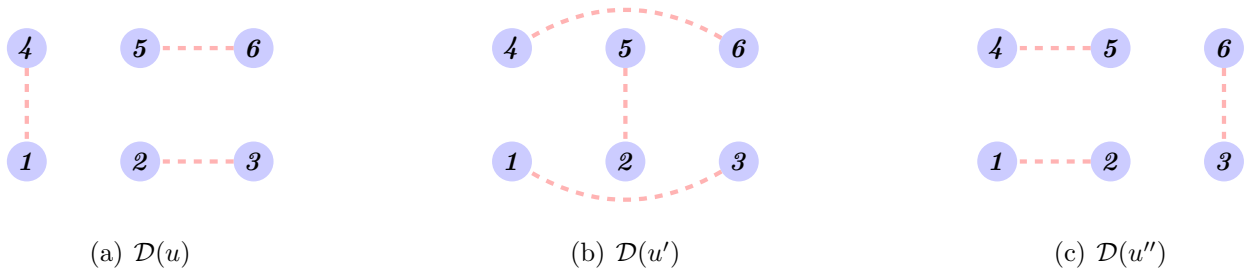
Figure 2: Example 2
