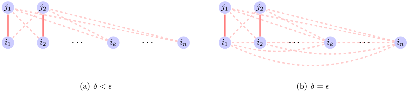
Figure 6: Example 5
