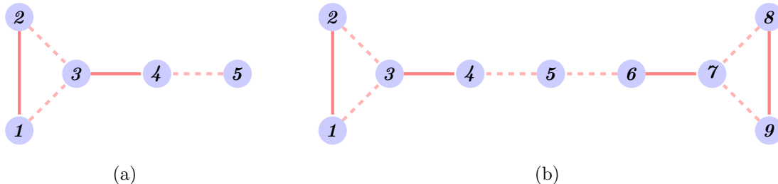
Figure 5: Example 4
